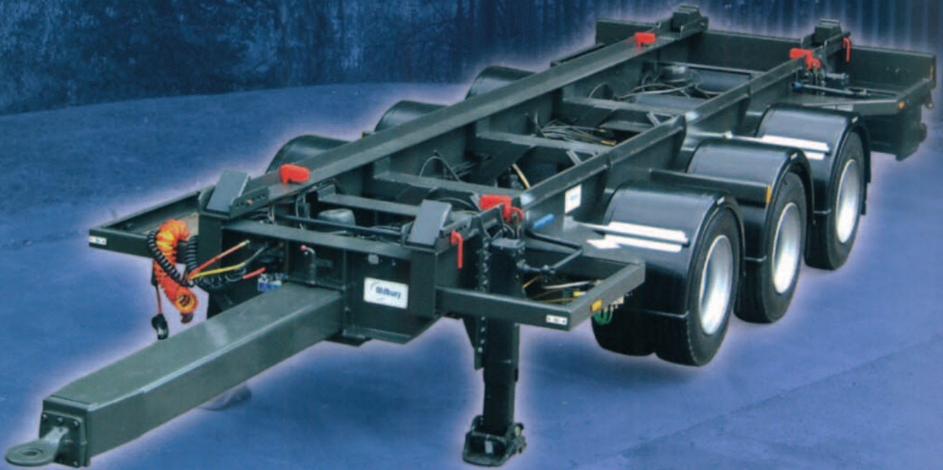
Hi-spec 24 tonne GTW showing light weight construction
